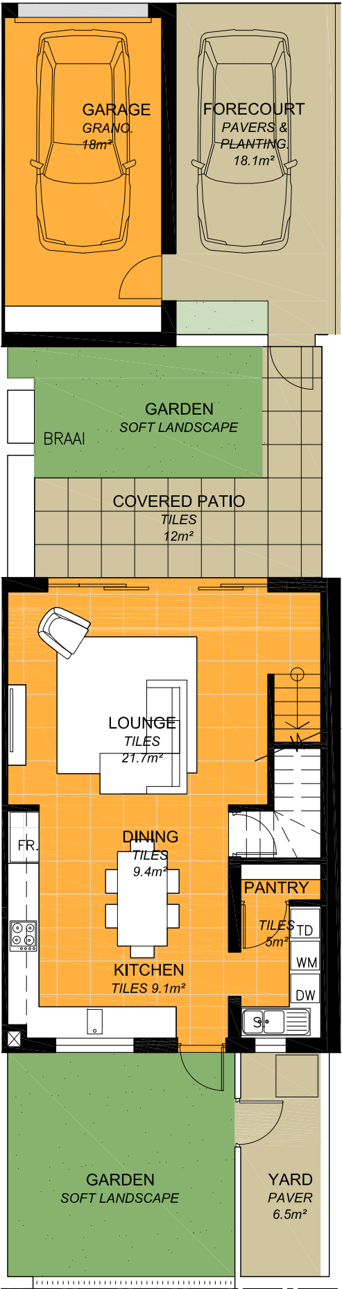
GROUND FLOOR
