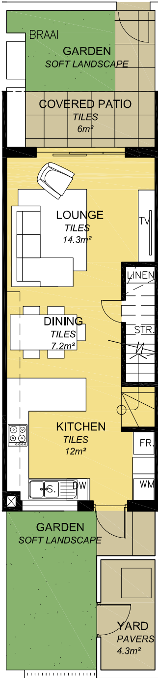
GROUND FLOOR
